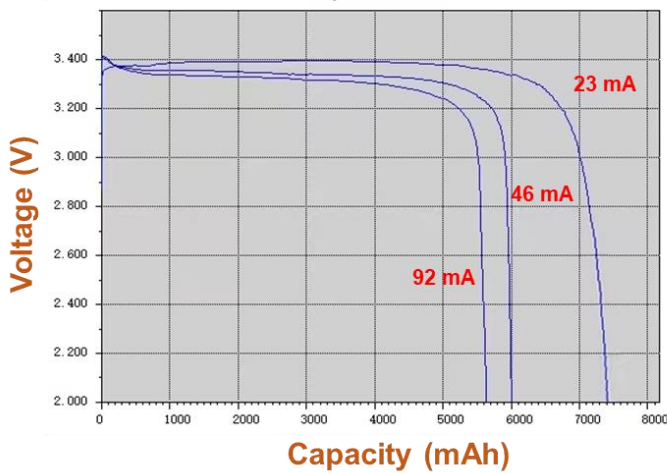
RT Capacity test at different rates
