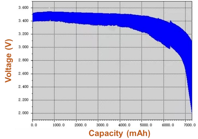
Pulse 59.0 s 40 mA 1.0 s 200 mA at 25 °C to 2.0 V
