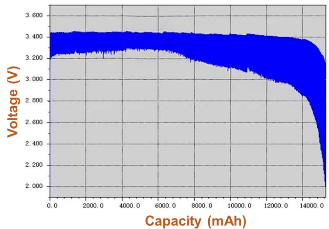
Pulse 59.0 s 23 mA 1.0 s 115 mA at 25 °C to 2.0 V
